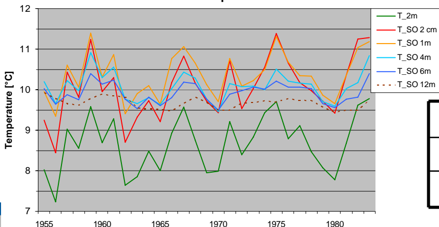
Annual mean temperature Potsdam
