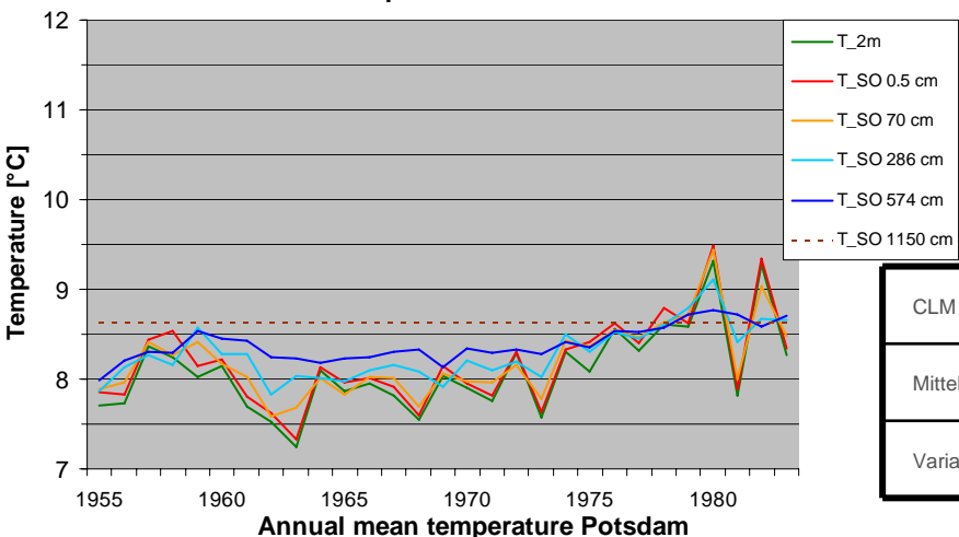
Annual mean temperature of CLM Simulation A1B
